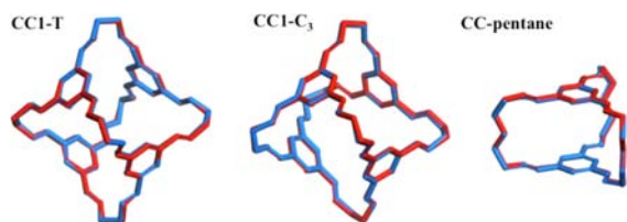
Figure 2. Overlay of X-ray structure (blue) and predicted structure (red) for CCI-T , CCI-C 3 , and CC-pentane . CCI-T = desolvated crystal structure; 8 CCI-C 3 = DCM solvate; 35 CC-pentane = methanol solvate prepared in this study. Further examples of predictions for published cages are given in Figure S6.
